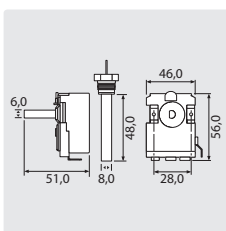
3/8" M. Contact 16 A - 380 V (AC1)
