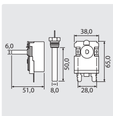
M14 x 1 M. Contact 16 A - 380 V (AC1)
